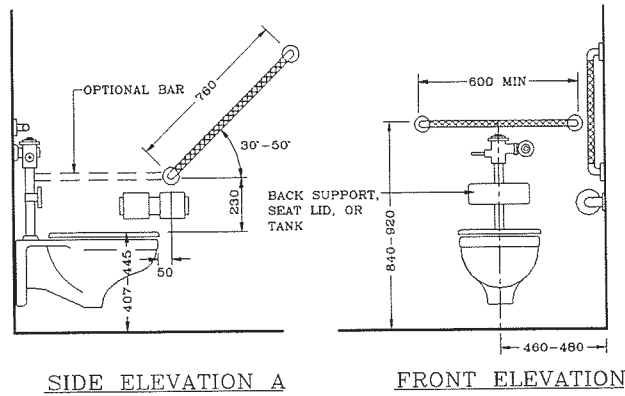
SIDE ELEVATION A
