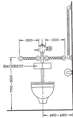
FRONT ELEVATION
