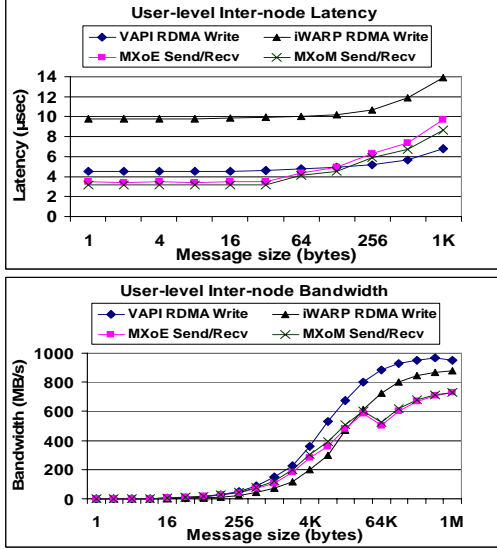
Figure 1. User-level ping-pong performance.
