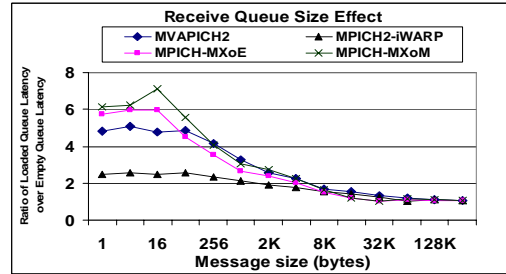
Figure 8. Effect of receive queue usage.
