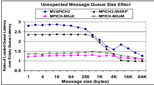
Figure 7. Effect of unexpected messages.
