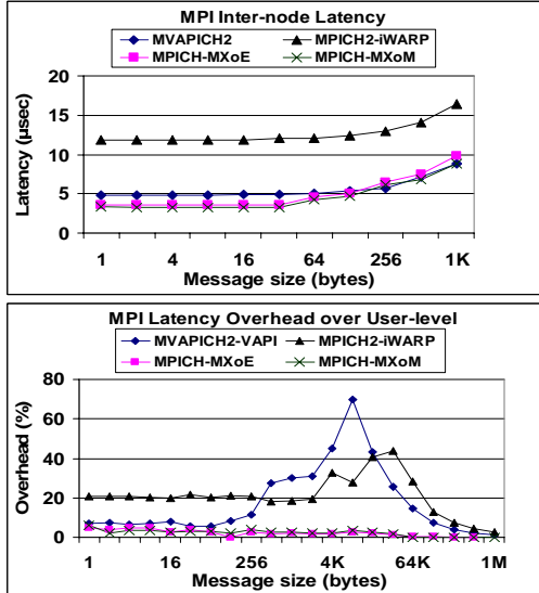
Figure 3. MPI ping-pong latency and its overhead over user-level.
