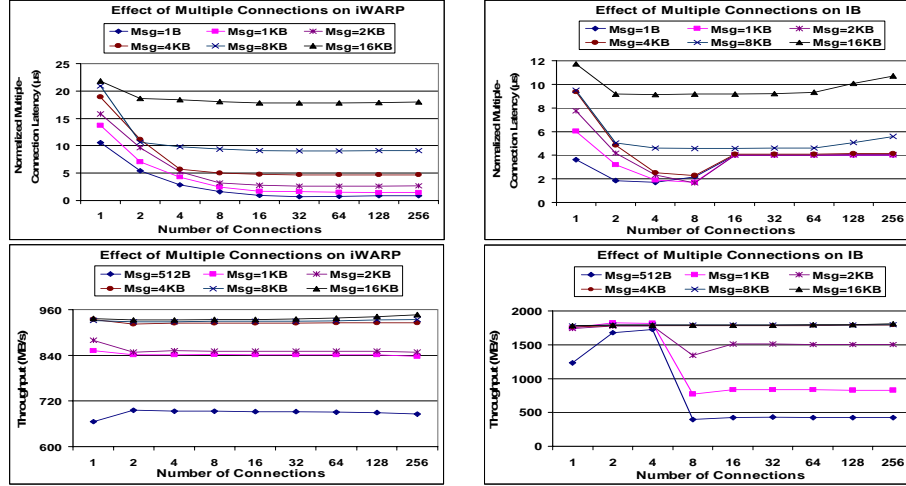
Figure 2. Throughput and normalized multiple-connection latency of NetEffect iWARP and Mellanox IB.
