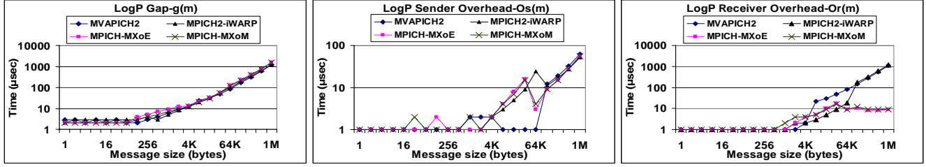
Figure 5. Parameterized LogP parameters.
