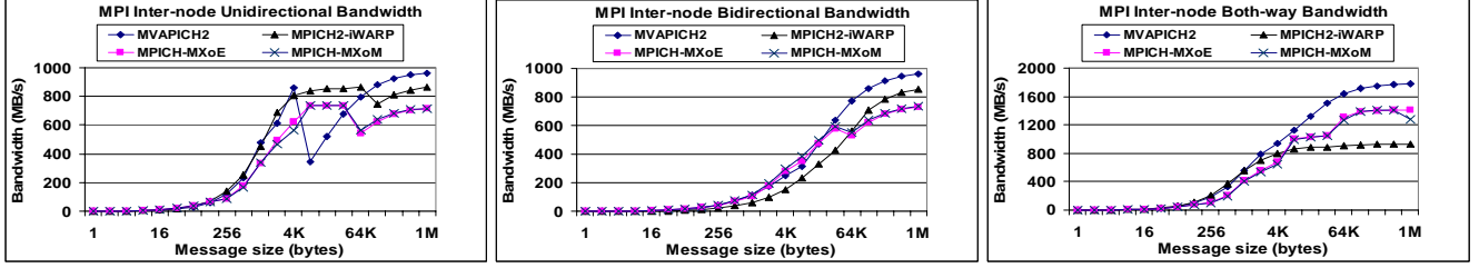
Figure 4. MPI bandwidth.
