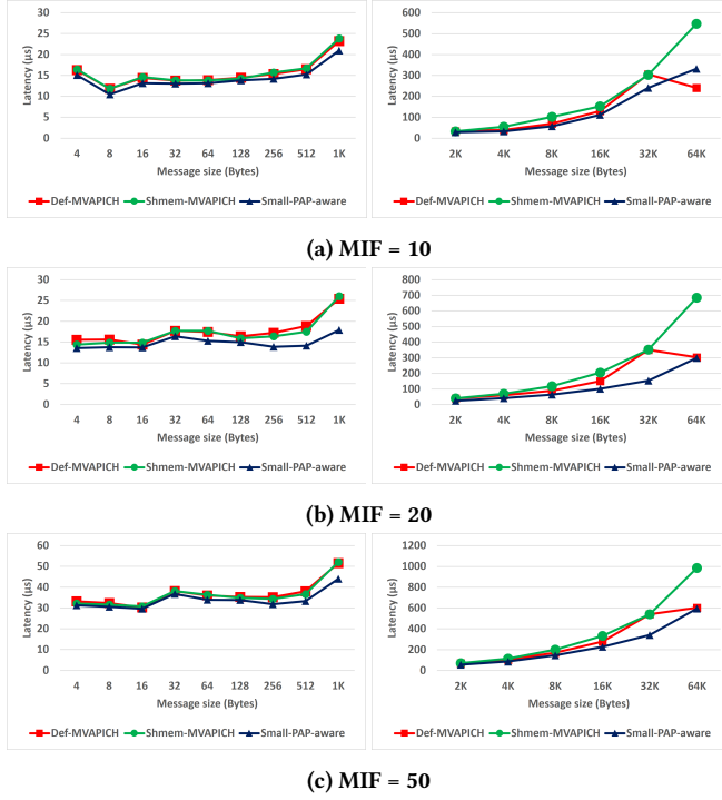
Figure 7: Comparison of the proposed Small-PAP-aware MPI_Allreduce against the Def-MVAPICH and shm-mem-MVAPICH algorithms under imbalanced workload, different MIFs and 32 processes on a single node on Cedar
