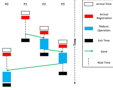
Figure 6: Example run of the proposed large message PAP-aware reduce algorithm for four processes
