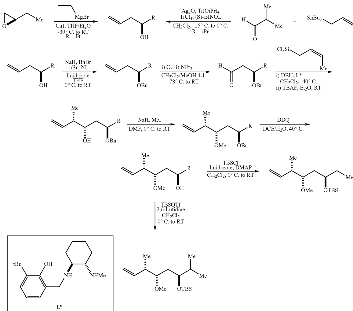
Scheme 1. Synthesis of tert-butyl(((3R,5S,6S)-5-methoxy-6-methyloct-7-en-3-yl)oxy)dimethylsilane and tert-butyl(((3S,5S,6S)-5-methoxy-2,6-dimethyloct-7-en-3-yl)oxy)dimethylsilane
