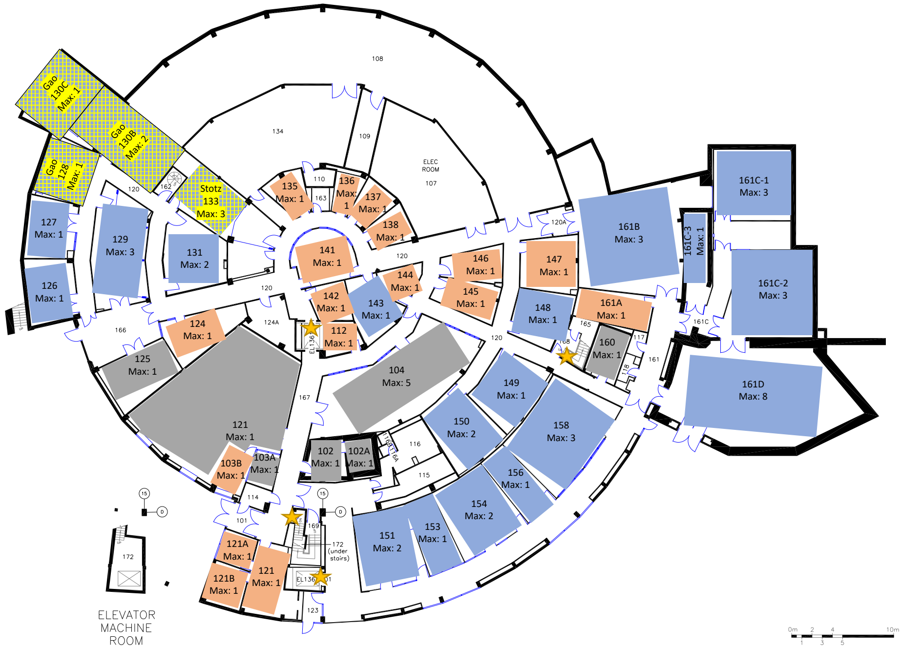
LEVEL 1 – FLOOR PLAN
